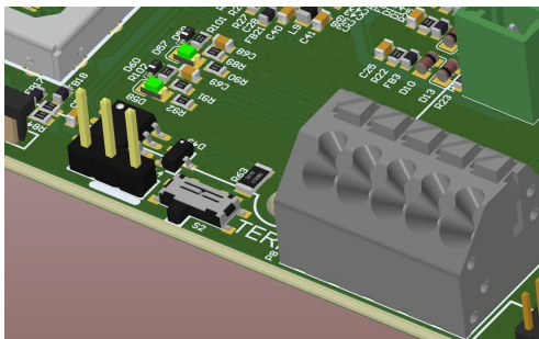
Fig. 25: The place of applying the terminating jumper (variant B)
