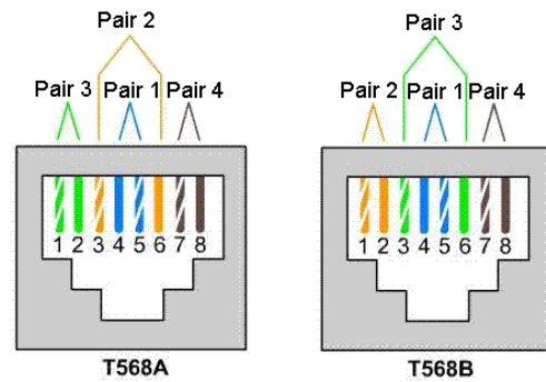
Fig. 26: Termination of the Ethernet cable according to TIA-568A/B to 100BaseT.
