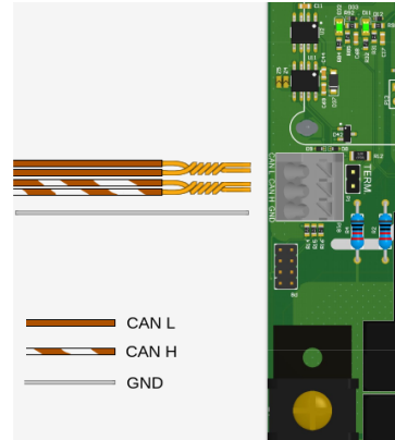
Fig. 18: Diagram of Enelion Chain communication cables connection (variant A)
