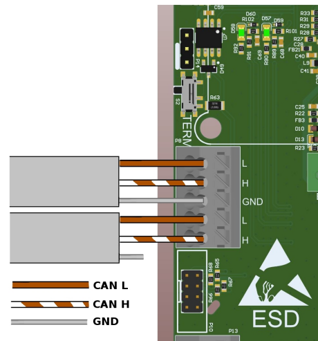
Fig. 19: Diagram of Enelion Chain communication cables connection (variant B)
