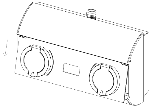
Fig. 7: Sliding the front panel from the device housing.
