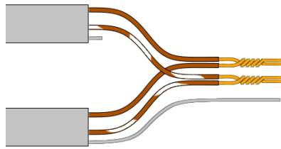
Fig. 16: Incoming and outgoing communication cable connection (variant A)
