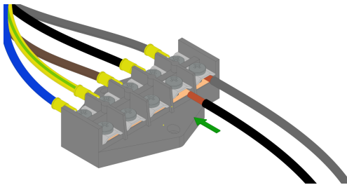
Fig. 15: Connection with solid conductors – wire.
