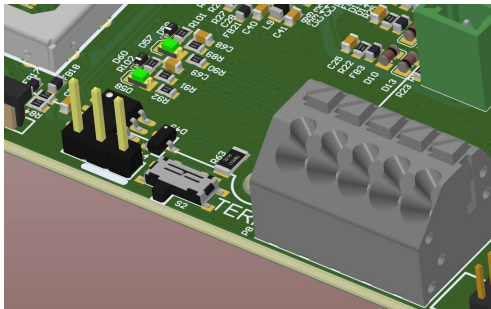
Fig. 22: The place of applying the terminating jumper (variant B)
