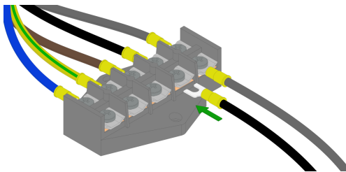
Fig. 14: Connection using fork terminals.
