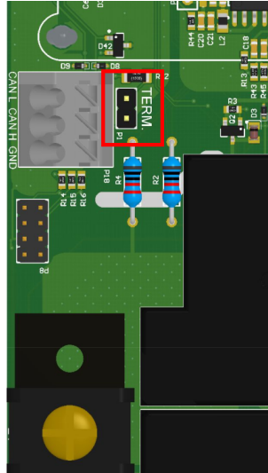
Fig. 21: The place of applying the terminating jumper (variant A)
