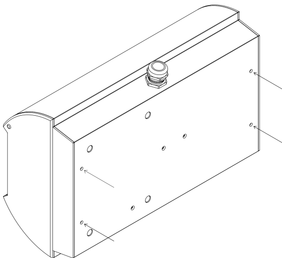
Fig. 11: Mounting holes of Enellion Wallbox Duo as seen from the back of the device.
