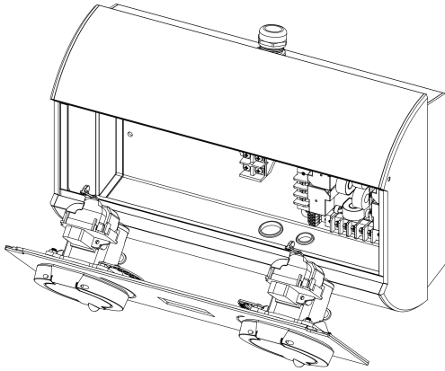
Fig. 9: The device open with the access to its interior.
