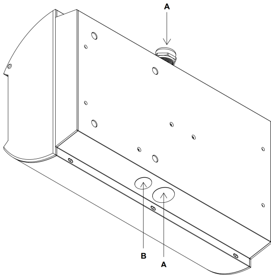
Fig. 12: Locations of cable entry points in Enelion Wallbox Duo.
