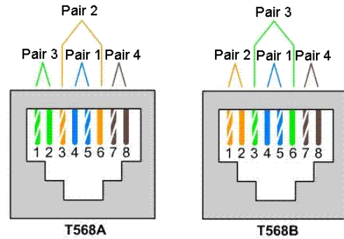
Fig. 23: Termination of the Ethernet cable according to TIA-568A/B to 100BaseT.
