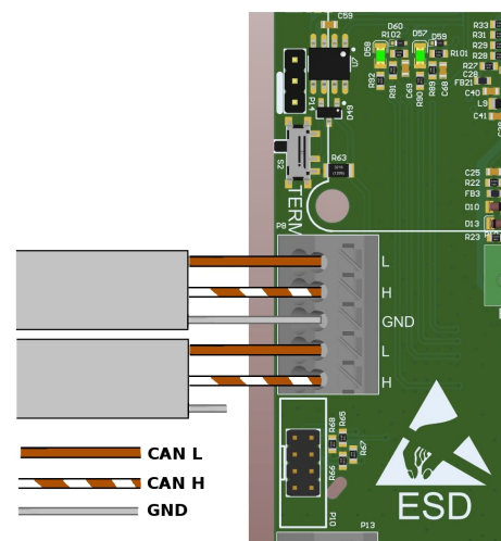
Fig. 26: Diagram of Enelion Chain communication cables connection (variant B)
