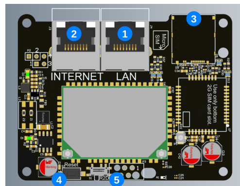
Fig. 31: Enelion Bridge module diagram.
