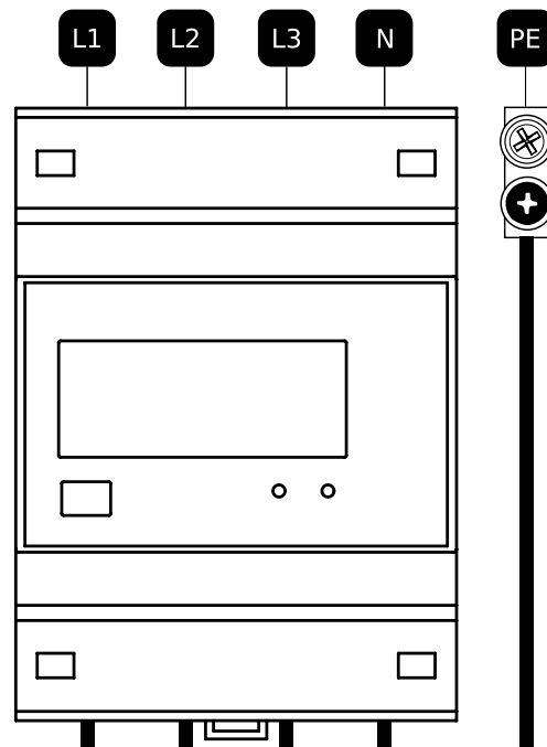
Fig. 22: Recommended connection when applying a MID meter.
