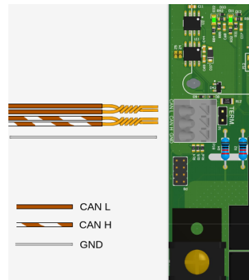
Fig. 25: Diagram of Enelion Chain communication cables connection (variant A)
