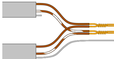
Fig. 23: Incoming and outgoing communication cable connection (variant A)
