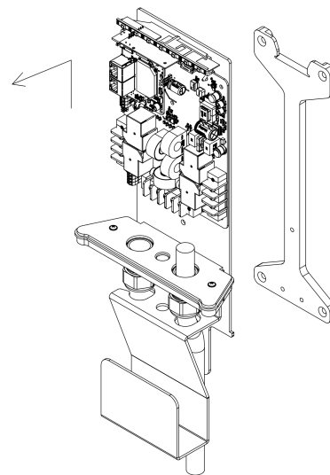
Fig. 8: Removing the device from the wall anchor.
