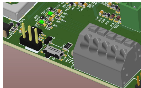
Fig. 23: The place of applying the terminating jumper (variant B)
