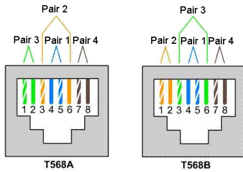
Fig. 24: Termination of the Ethernet cable according to TIA-568A/B to 100BaseT.
