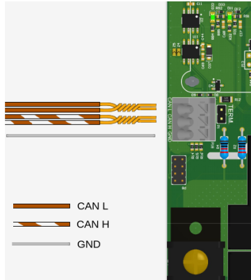
Fig. 19: Diagram of Enelion Chain communication cables connection (variant A)
