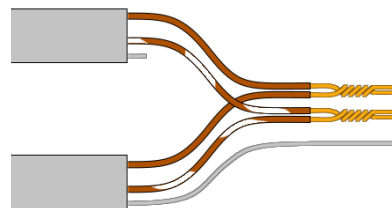
Fig. 17: Incoming and outgoing communication cable connection (variant A)
