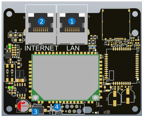
Fig. 25: Enelion Bridge module diagram.
