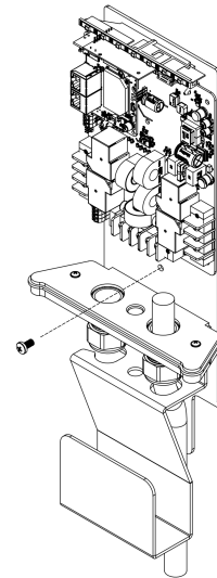
Fig. 7: Removing the anchor bolt.
