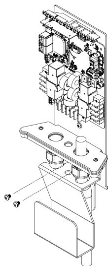
Fig. 6: Removing the charging cable hold.
