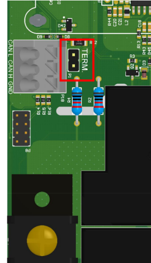
Fig. 22: The place of applying the terminating jumper (variant A)
