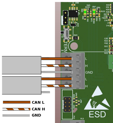
Fig. 20: Diagram of Enelion Chain communication cables connection (variant B)
